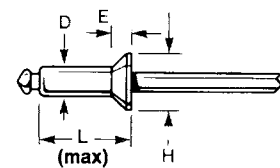
120° Countersunk Head
