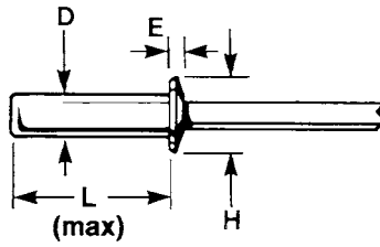
Dome Head
