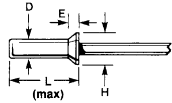
120° Countersunk Head
