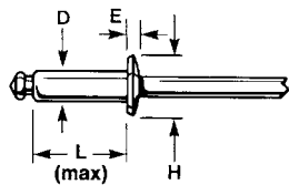
Dome Head
