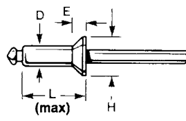
120° Countersunk Head
